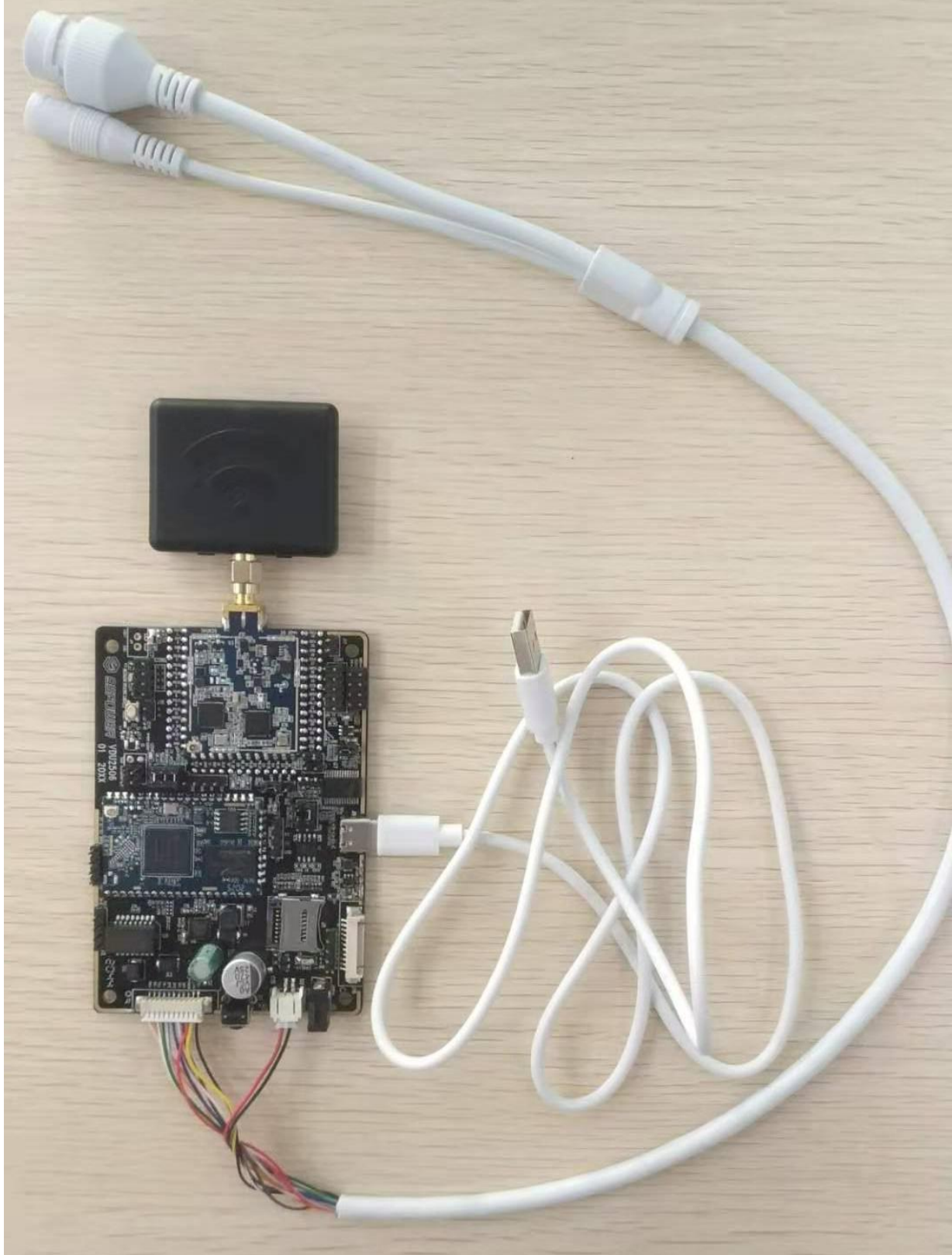
Figure 1.3 :SKU623 EVB (Fully-configured version)
