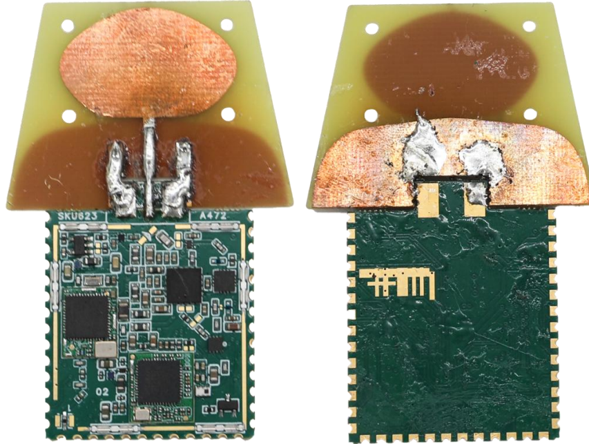
Figure 1.2 :SKU623-P with PCB soldering Antenna
