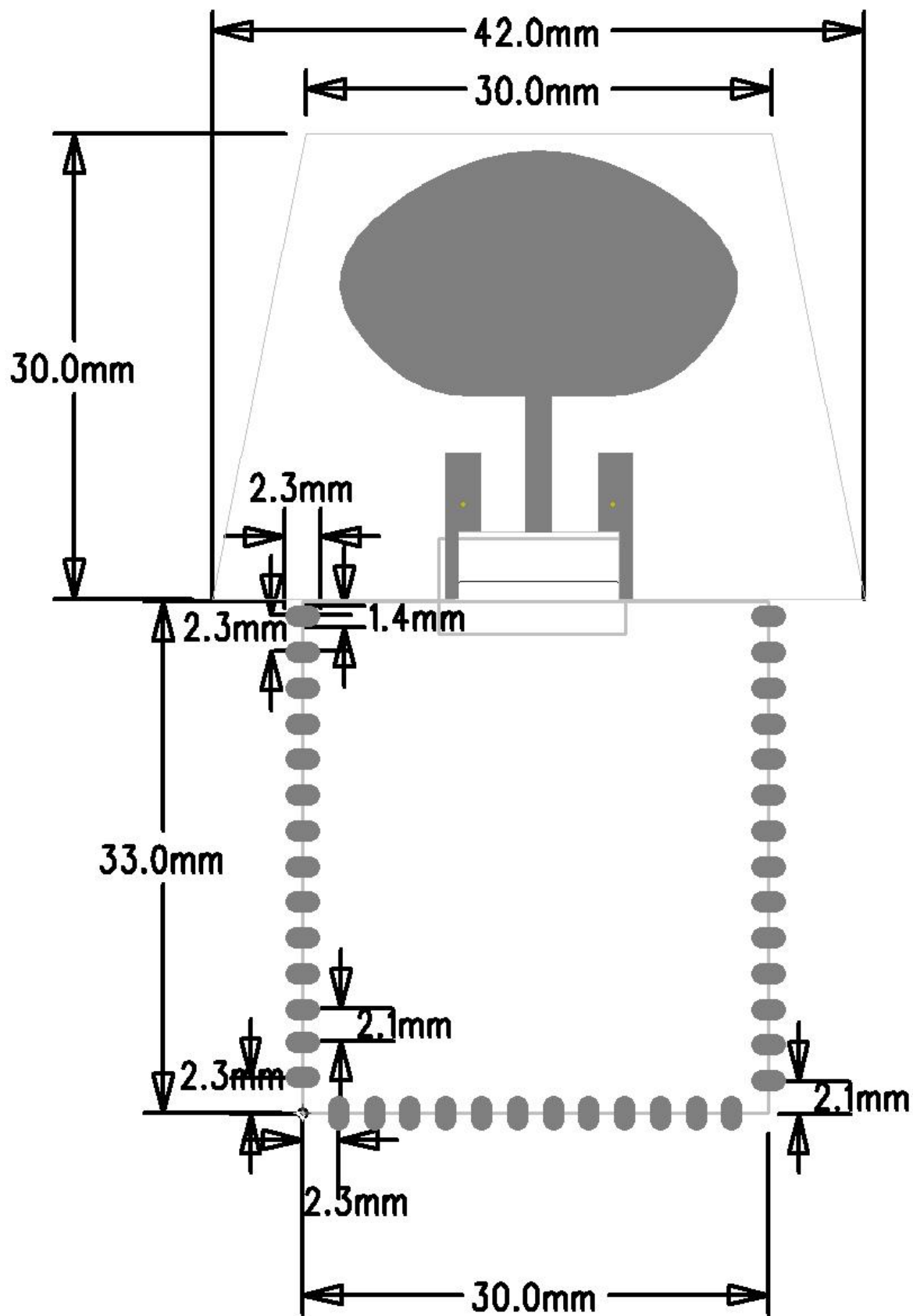
Figure 8-1: SKU623 PCB Footprint and Dimensions(units: mm)
