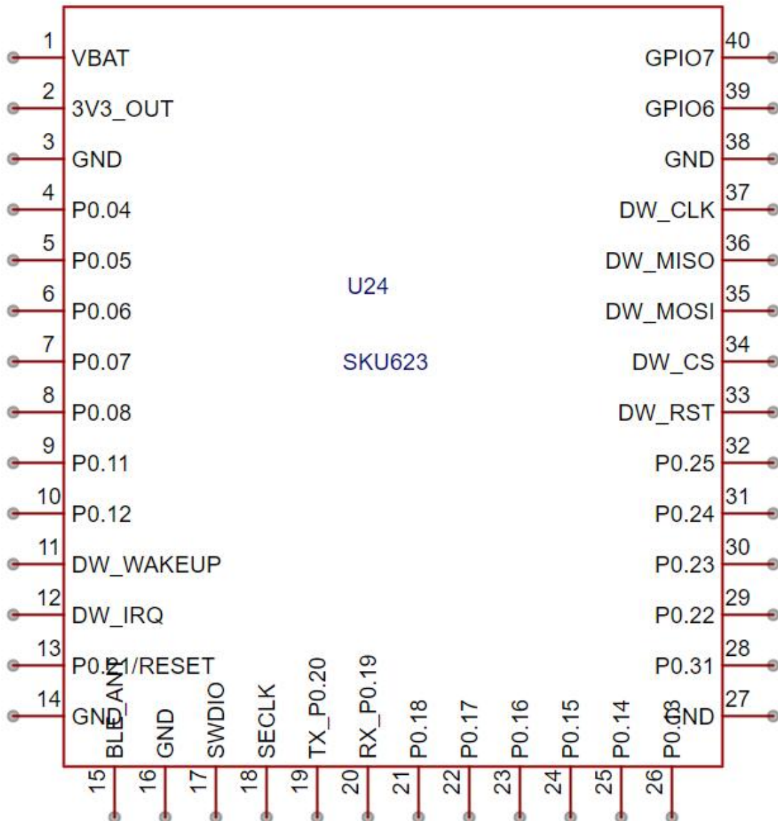
Figure 6-1: SKU623Module Pinout (TOP View)
