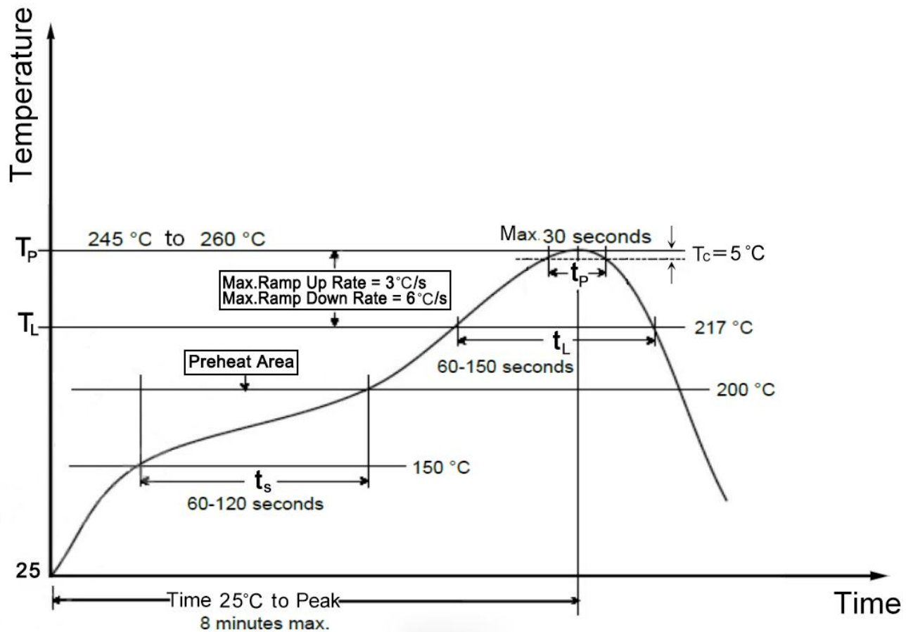
Figure 9-1: SKU623 Typical Lead-free Soldering Profile 无铅回流焊接炉温曲线
